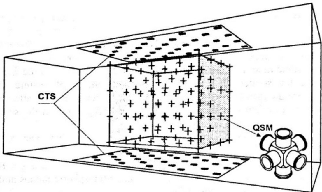
Figure 1. Schematic view of NEVOD-91 setup with 91 QSM and 2 \times 32 scintillation counters
