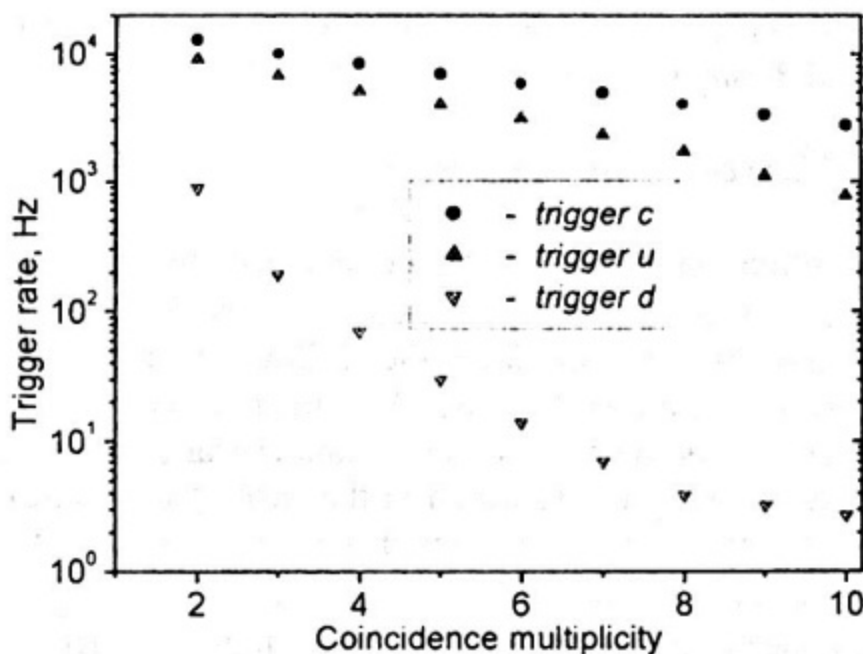
Figure 2. Dependence of trigger rate on coincidence multiplicity
