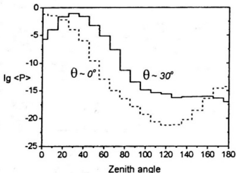
Figure 6. Examples of averaged probability functions P(\theta) calculated for a vertical muon and an inclined one (arb. units).
