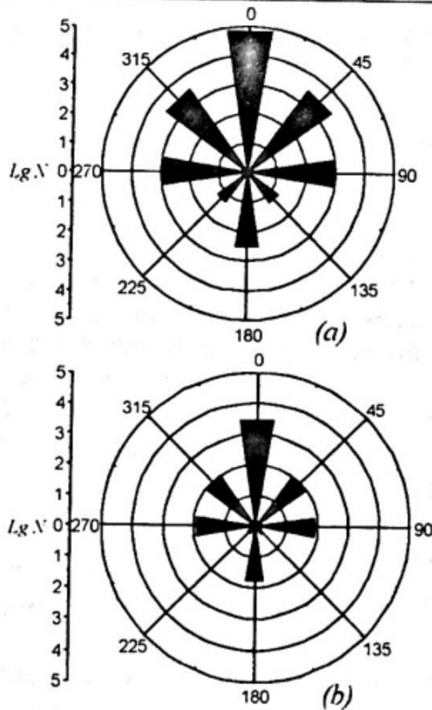
Figure 5. Azimuth diagrams of measuring module response: (a) combinations with up-looking hit PMT. (b) with down-looking hit PMT
