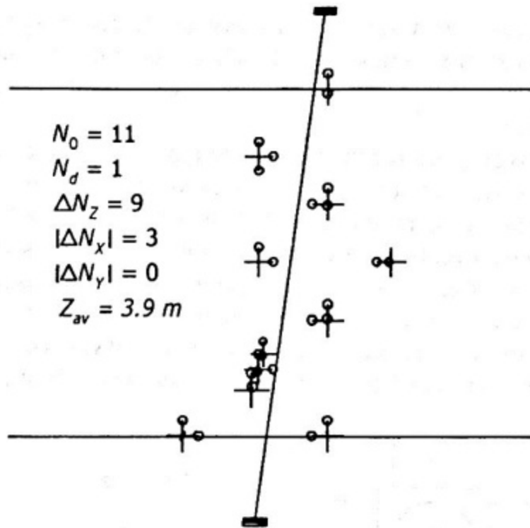
Figure 3. Vertical muon event selected by calibration telescope. Hit phototubes are marked by the circles
