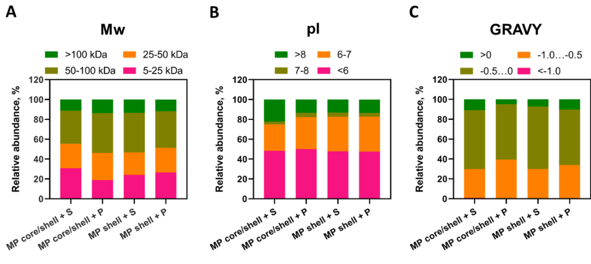
Figure 4. Relative label-free quantification intensities of proteins grouped according to their (A) molecular weights (Mw), (B) isoelectric points (pI), and (C) grand average of hydropathicity (GRAVY) scores adsorbed on core/shell and shell MPs upon their incubation with serum or plasma. The Mw, pI, and GRAVY were calculated on the basis of the primary sequences of the proteins using the ProtParam software.
