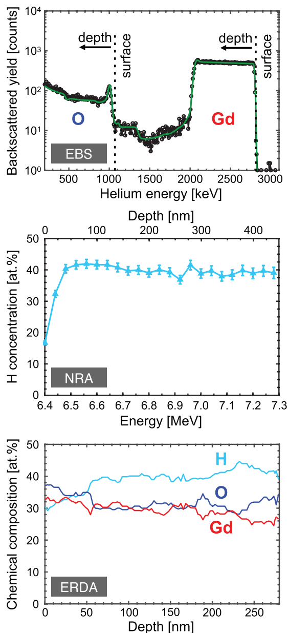
Figure 1. Ion beam analysis including elastic backscattering spectrometry (EBS), nuclear reaction analysis (NRA), and coincidence time-of-flight elastic recoil detection analysis (ERDA). Depth profile values in nanometers were calculated using the measured areal density as well as the film thickness.
