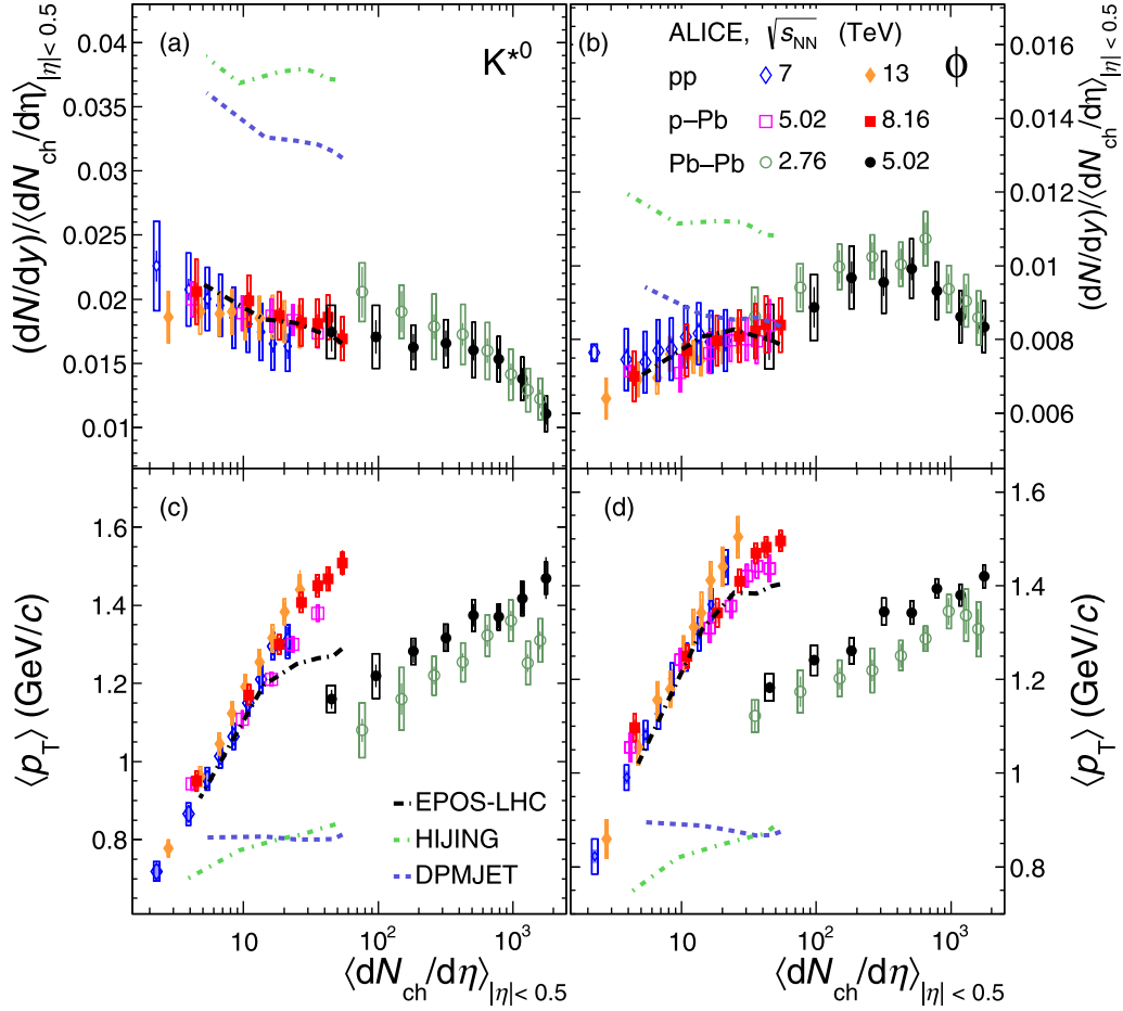
FIG. 5. The multiplicity-scaled integrated yield ((dN/dy)/(\langle dN_{ch}/d\eta \rangle_{|η|<0.5})) (upper panels) and mean transverse momentum (\langle p_T \rangle) (bottom panels) for K^{*0} (left panels) and \phi (right panels) as a function of \langle dN_{ch}/d\eta \rangle_{|η|<0.5} measured in the ALICE central barrel in pp collisions at \sqrt{s} = 7, 13 TeV, in p -Pb collisions at \sqrt{s_{NN}} = 5.02, 8.16 TeV, and Pb-Pb collisions at \sqrt{s_{NN}} = 2.76, 5.02 TeV. Measurements are compared with the predictions from EPOS-LHC [31,69], DPMJET [32], and HIJING [33] for p -Pb collisions at \sqrt{s_{NN}} = 8.16 TeV. Statistical uncertainties are represented as bars, boxes indicate total systematic uncertainties.
