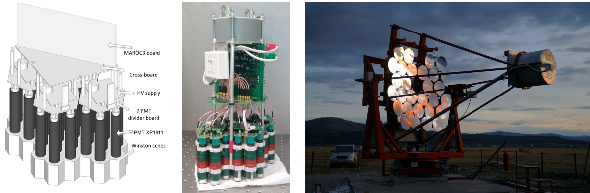
Figure 11. Left and center: Design and photo of a TAIGA-IACT camera cluster, which contains 28 PMTs and an independent board generating the trigger. Right: Photo of the first TAIGA-IACT telescope with 29 mirror segments installed.
