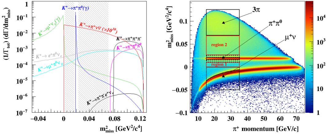
Fig. 2. Left: true m^2_{\text{miss}} distribution of the K^+ \rightarrow \pi^+ \nu \pi^0 decay and the main K^+ decays, computed under \pi^+ mass hypothesis for the charged particle in the final state. Signal (red) is multiplied by 10^{10} for visibility and the dashed areas show the signal search regions. Right: reconstructed m^2_{\text{miss}} as a function of \pi^+ momentum for control events selected without applying \pi^+ identification and photon rejection. Signal regions 1 and 2, as well as the 3\pi , \pi^+\pi^0 and \mu^+\nu background regions are also shown. The control regions located between the signal and background regions are indicated by dashed lines.
