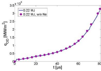
Figure 3. Intra-ELM power loads at the outer divertor during ELM duration ( \sim 80 \mu\text{s} ) with and without Ne seeding
