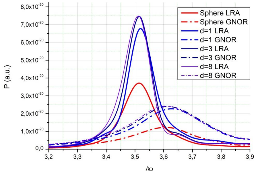
Figure 3. EEL spectra obtained for single Ag sphere (red lines) and dimers of Ag spheres, a=2nm . Electron kinetic energy 50 keV, b_x=2.3nm , b_y=0 . Gap size d (nm) varies.
