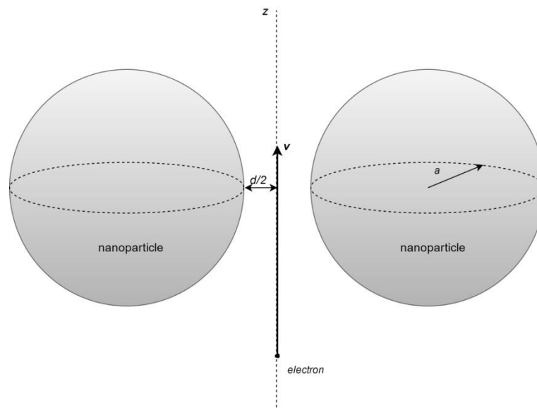
Figure 4. EELS problem geometry for electron beam passing through the gap.
