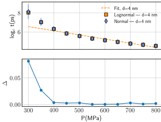
Fig. 4. Top: Mean values of the closing time versus the applied pressure for the 4 nm void at 1250 K. The squares represent the mean values which derive from a log-normal fitting of the raw data, while the diamonds from a fitting to a normal distribution. Bottom: Difference of the mean values between log-normal and normal distribution.
