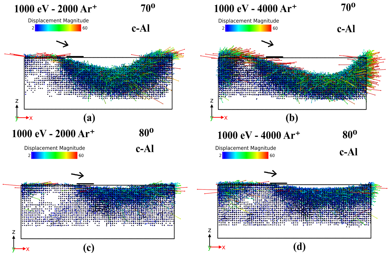
FIG. 7: c-Al cell after 1 keV \text{Ar}^+ (a) 2k impacts and (b) 4k impacts at 70^\circ ; and after (c) 2k impacts and (d) 4k impacts at 80^\circ . Only those displacements greater than 2 Å are presented and the displacement vectors are scaled by a factor of 0.3 for a better visualization. The initial impact region is marked in black.
