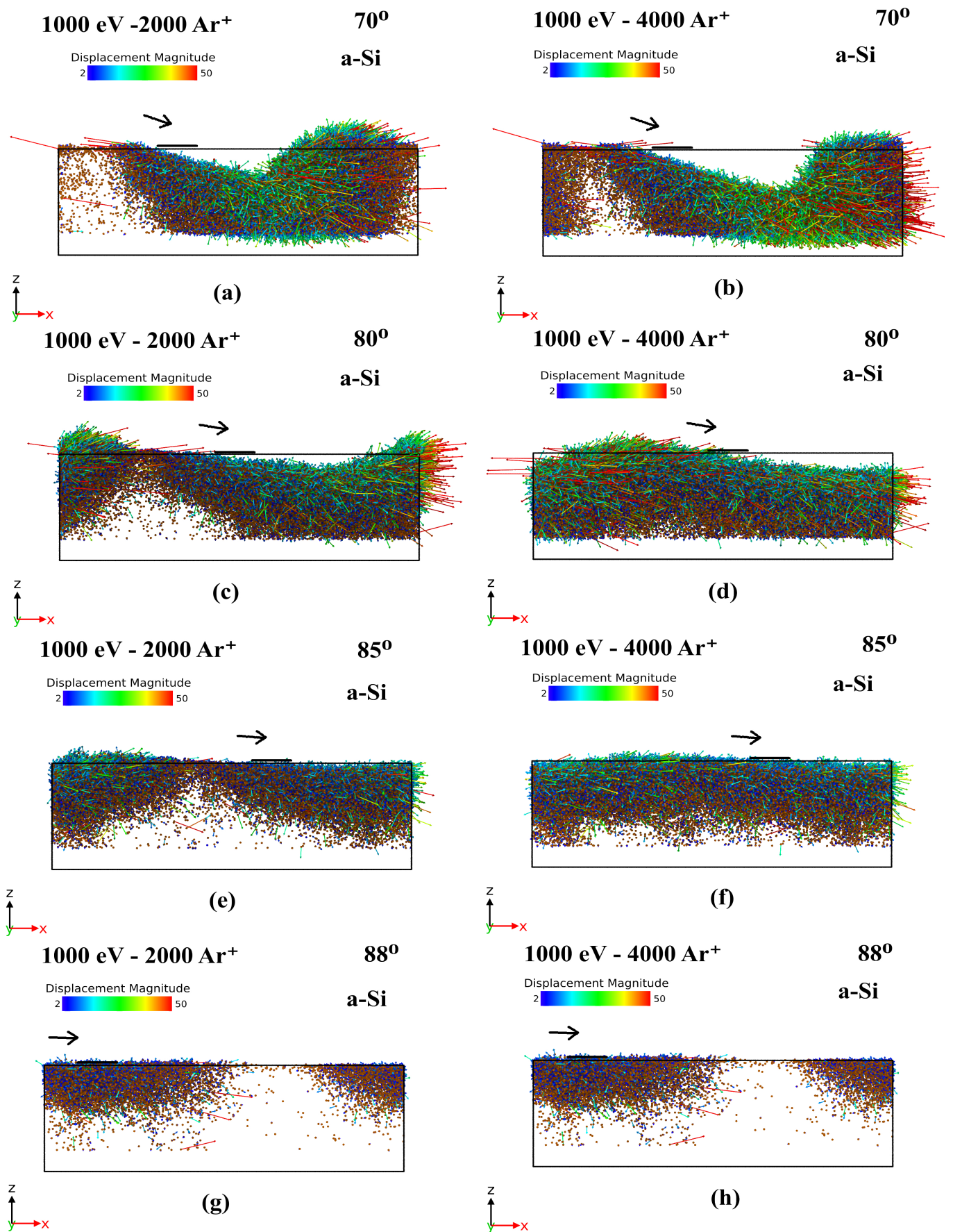
FIG. 4: a-Si cell under 1000 eV \text{Ar}^+ after (a) 2k impacts and (b) 4k impacts at 70°; after (c) 2k impacts and (d) 4k impacts at 80°; after (e) 2k impacts and (f) 4k impacts at 85°; and after (g) 2k impacts and (h) 4k impacts at 88°. Only displacements greater than 2 Å are presented and the displacement vectors are scaled by a factor of 0.3 for a better visualization. The initial impact region is marked in black.
