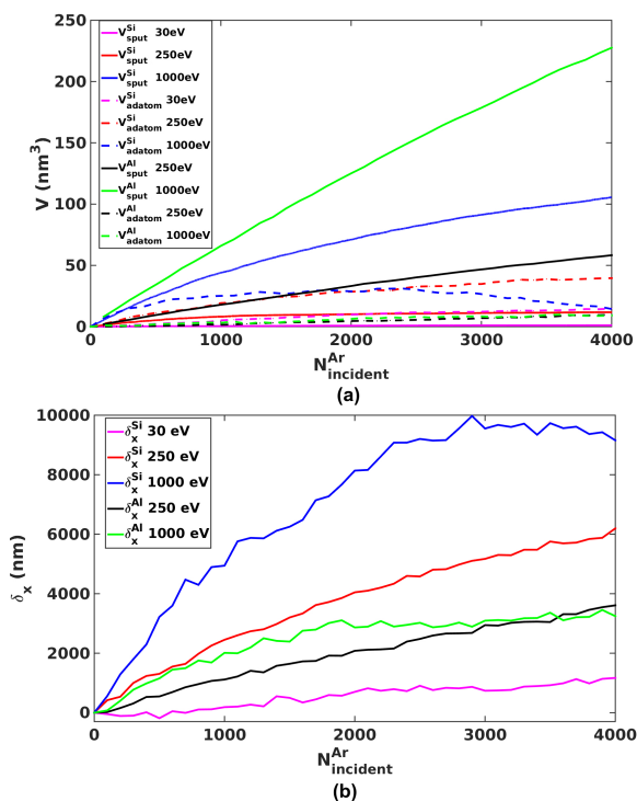
FIG. 12: Evolution of (a) the volume created by the sputtered atoms and adatoms and (b) the accumulated displacement in the x direction for 30 eV (from Ref. 13), 250 eV and 1000 eV \text{Ar}^+ for a-Si and for 250 and 1000 eV \text{Ar}^+ for c-Al at 70^\circ .
